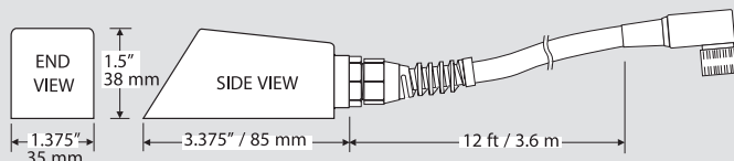
PSE4 ULTRASONIC DOPPLER SENSOR
